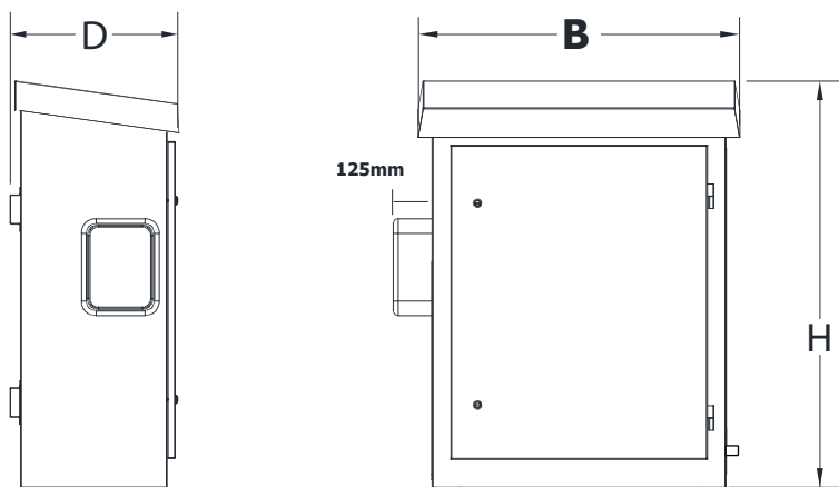
Fig 1 – IP54 kapslingsdimension
